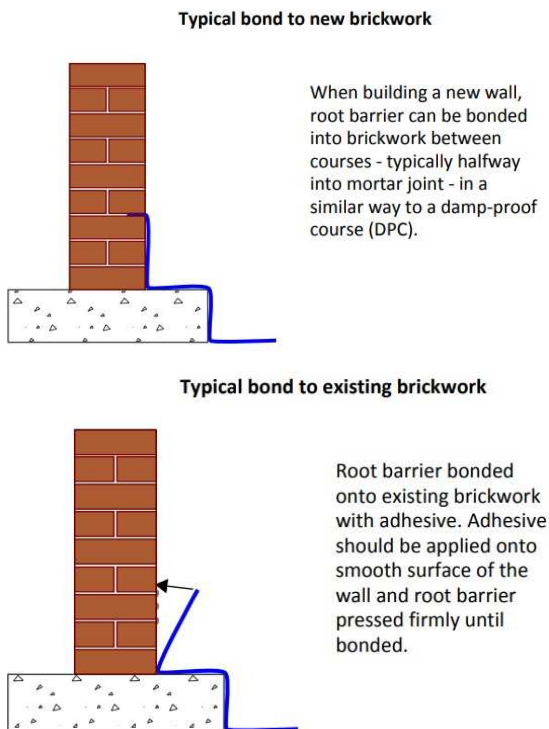
Fig 3: Bonding to walls or structures
